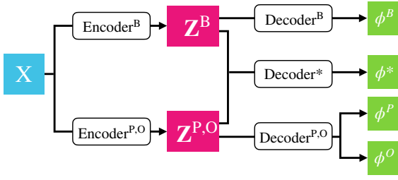
Fig. 4. Network architecture.
